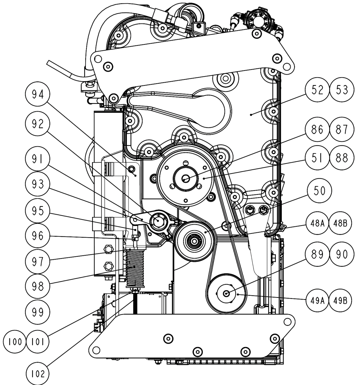
BOTTOM VIEW
