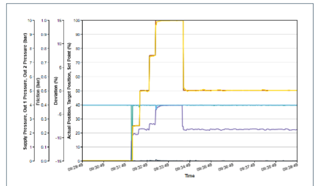
Online monitoring
