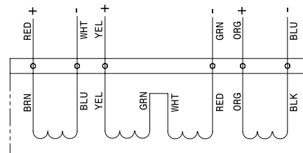
ELECTRICAL SCHEMATIC
