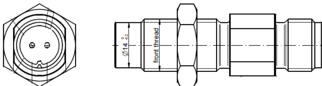
Figure 3. Schematic Diagram
