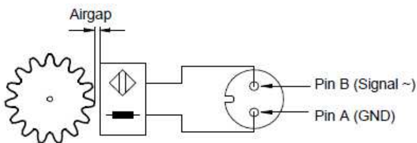
Figure 3. Schematic Diagram
