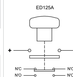
Connection Diagram
