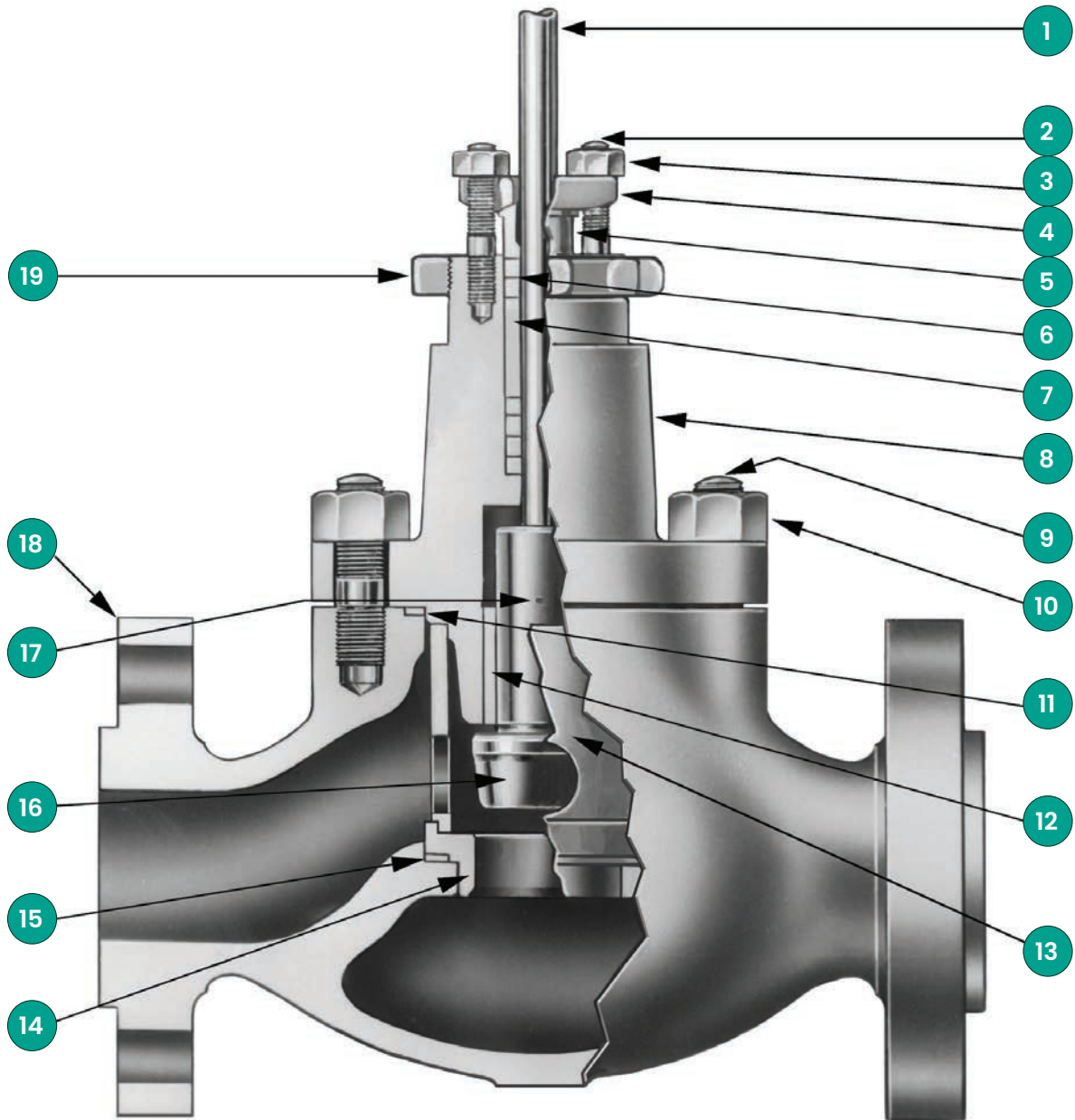
21000 Series - Standard Design
