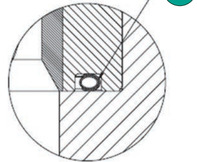
Flow-to-Open Seat-Ring Gasket Detail
