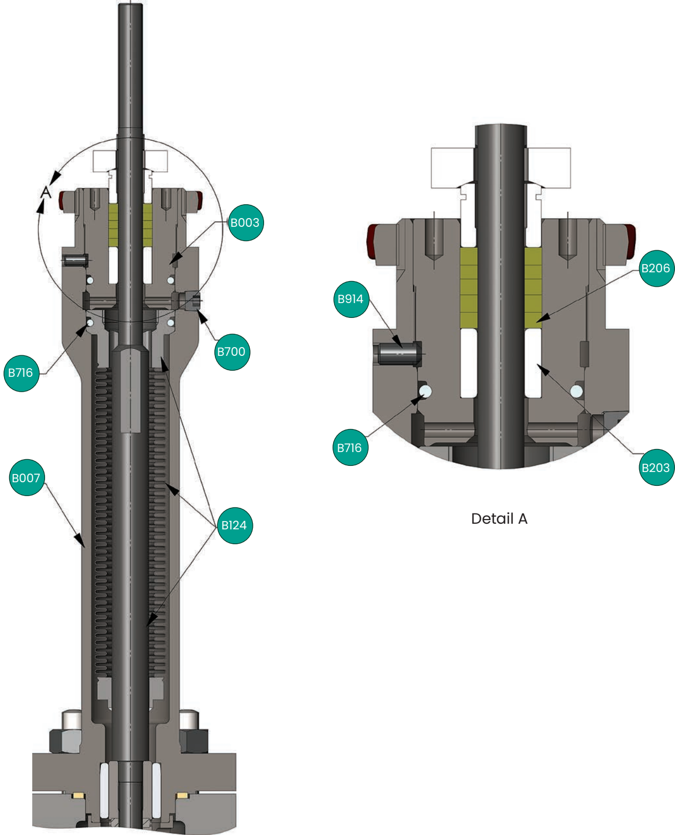
21000 BS Series Bonnet-less Design - 0.75" to 4"
