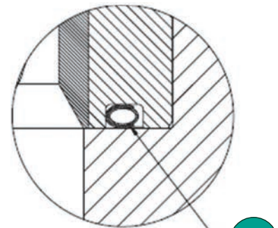
Flow-to-Close Seat-Ring Gasket Detail
