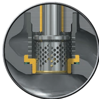
Double Stage Lo-dB and Anti-Cavitation Trim
