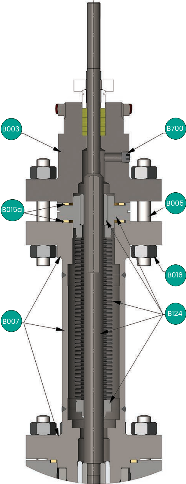
21000 BS Series Bonnet Design - 6"
