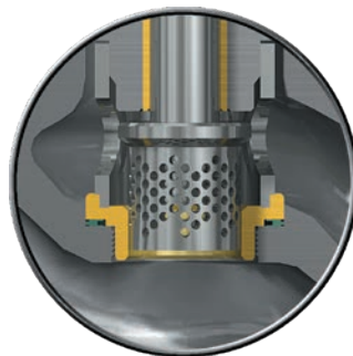
Single Stage Lo-dB and Anti-Cavitation Trim
