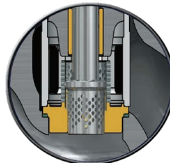
Double Stage Seat Extension Trim
